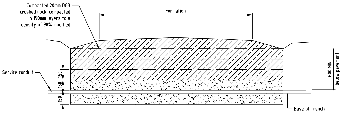
Backfilling Requirements for Open Trenching Under Unsealed Road Pavement Not to Scale
